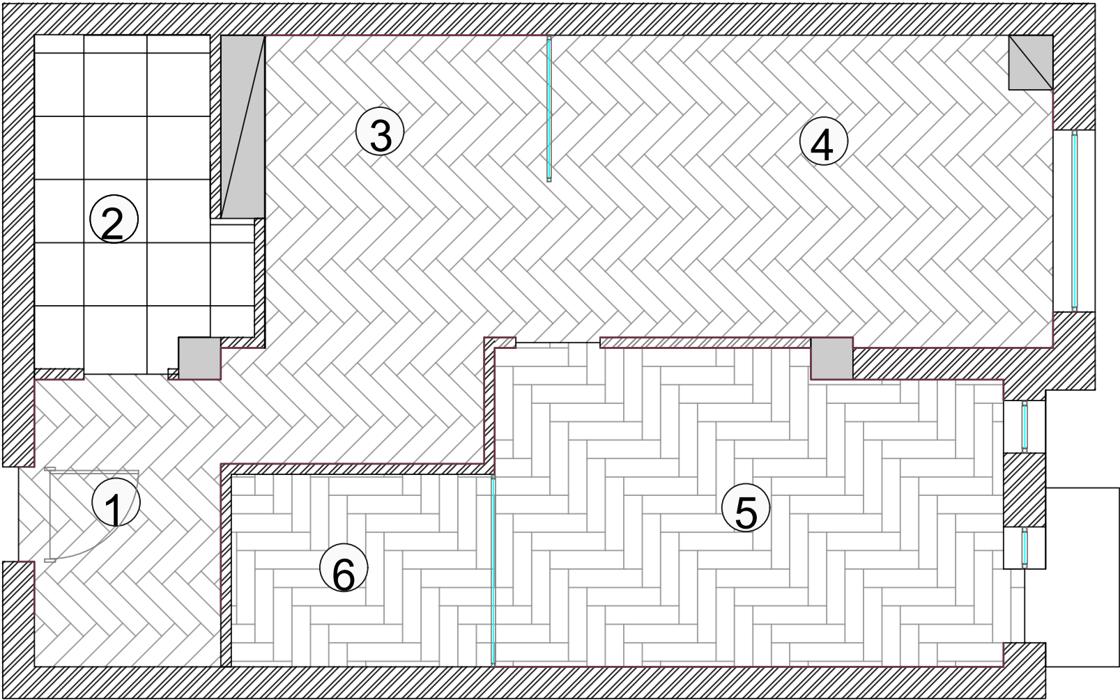
Parchet Herringbone – finisaj natur/ton cald (ex. Stejar Sardinia / Polar / Praline) – model oase de pește, 12 mm, clasa AC6/33
